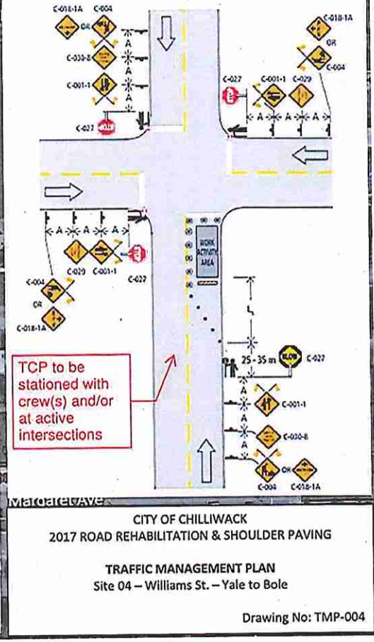
Figure 11.2: Intersection Lane Closure – Two-Lane, Two-Way Roadway with TCPs (Near Side) – Short and Long Duration
